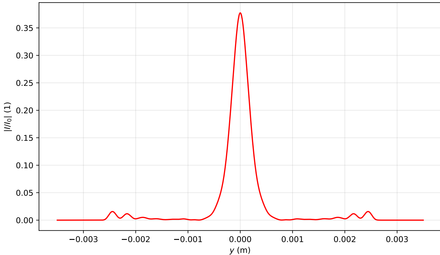
Intensity profile I(x=0, y, z=1.911)/I_0 , P_{in}=6.0P_{cr} , artificial time
